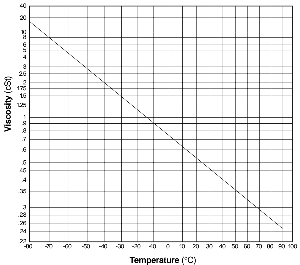
Fluorinert Liquid FC-84 Viscosity (cSt) vs. Temperature (°C)
